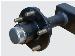
Standard 5 bolt hubs with high-speed bearings
